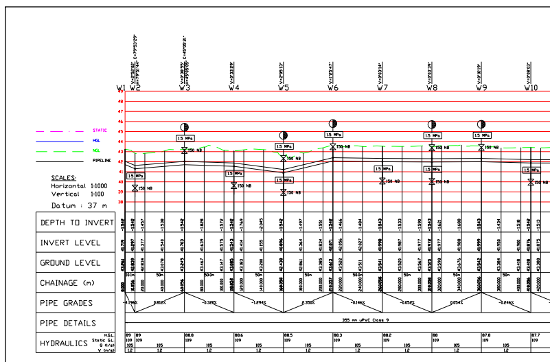
Fully detailed Longitudinal Section
