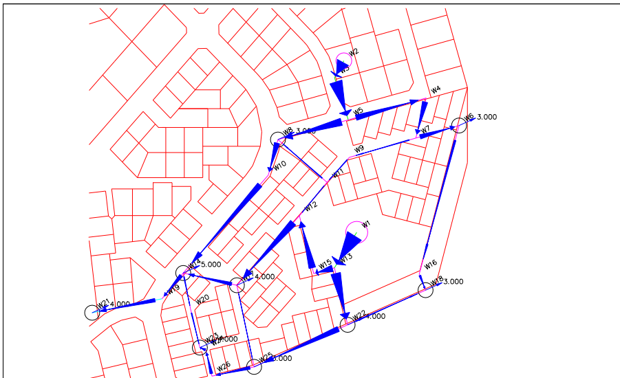
Graphical visualisation of pipe flows/velocities in plan
