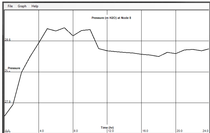
Simulation time-pressure graph for a node
