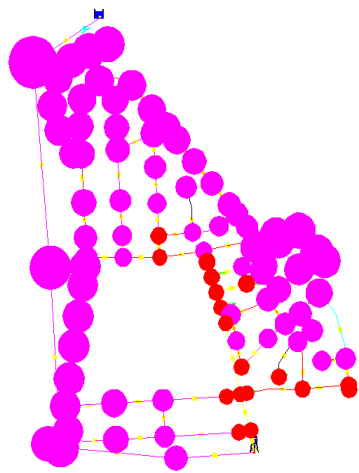
Graphical visualisation of node working pressures showing low pressure nodes in red.
