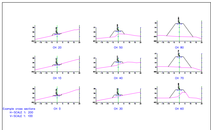
Figure 2 - Cross sections produced automatically
