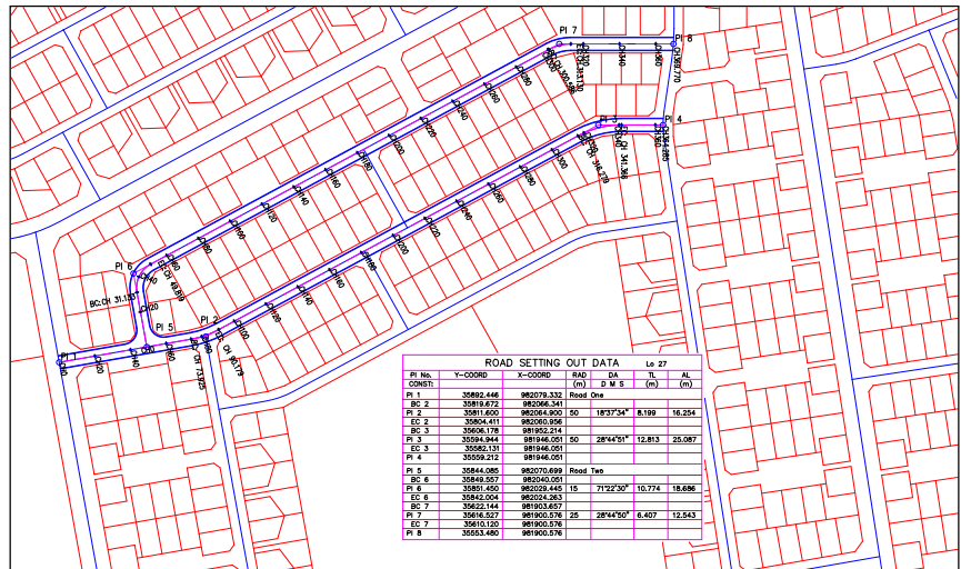
Figure 1- Road layout and setting out data produced automatically
